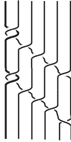
FIGURE 14. braid T_{6,2} .
