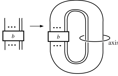
FIGURE 13. braid b \rightarrow braided link br(b) .
