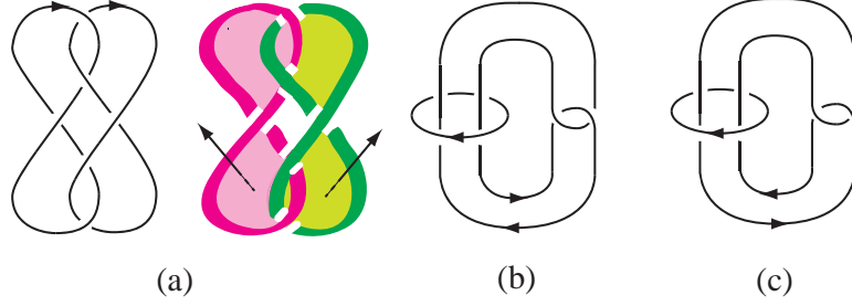
FIGURE 11. projections of the Whitehead link. [the minimal representatives of \overline{\mathbf{a}}_1 and \overline{\mathbf{b}}_1 are illustrated in (a).]
