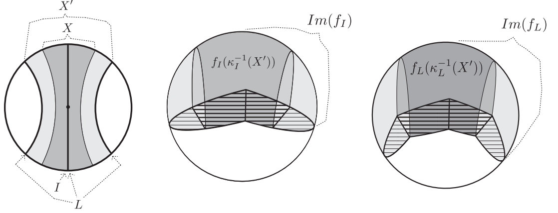
FIGURE 5. A basic example for Lemma 3.9.
