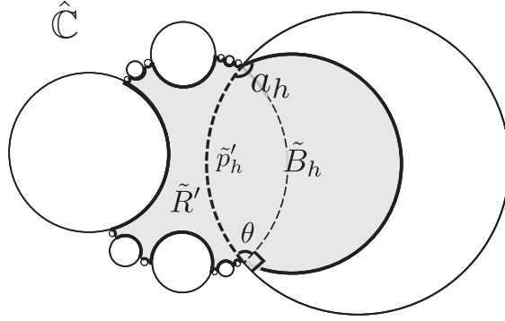
FIGURE 14. \mathcal{R}(\tilde{C}, \tilde{R}') = \tilde{R}' and \tilde{B}_h in C(L_P)
