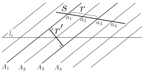
FIGURE 7. A case that p = 4 and q = 1 .
