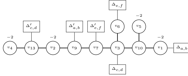
FIGURE 17. Dual graph
