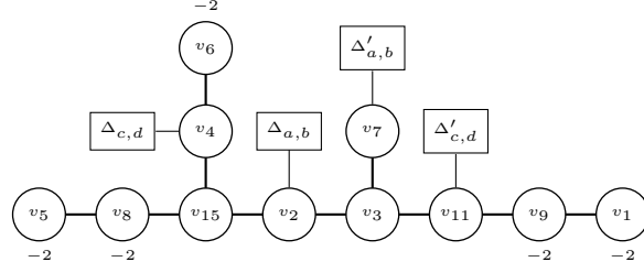
FIGURE 22. Dual graph
