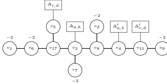
FIGURE 19. Dual graph
