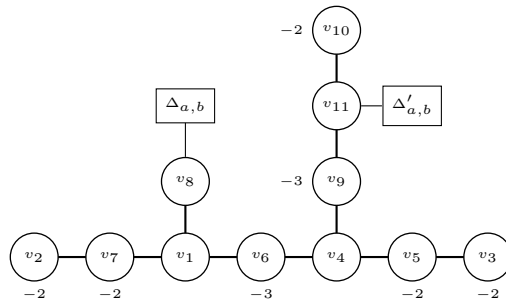
FIGURE 24. Dual graph
