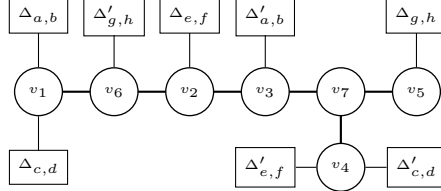
FIGURE 14. Dual graph
