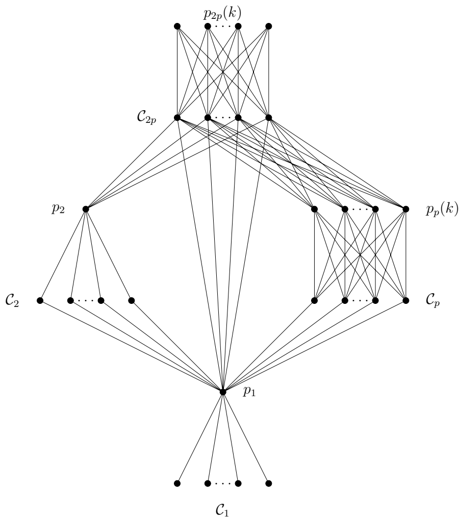
Figure 2: The boundary of \mathcal{F}_{L_{2p^2}}(\Gamma_{2p^2})^*
