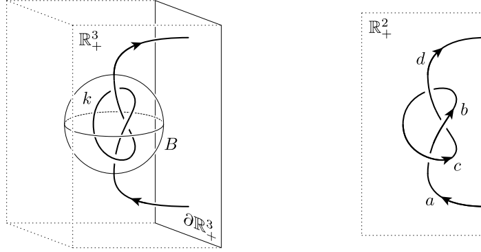
FIGURE 2. An oriented knotted arc k called the long trefoil and a 3-ball B which wholly contains the knotted part of k (left), and a diagram of k (right)
