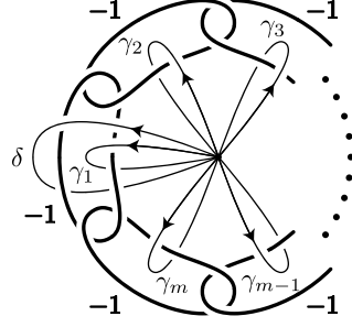
FIGURE 3. A surgery description of a fiber of \tau^m 3_1 (thick lines) and typical elements of G_m (thin lines)
