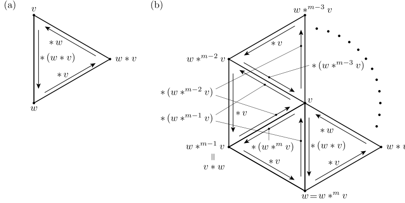
FIGURE 4. Some elements of X form triangles
