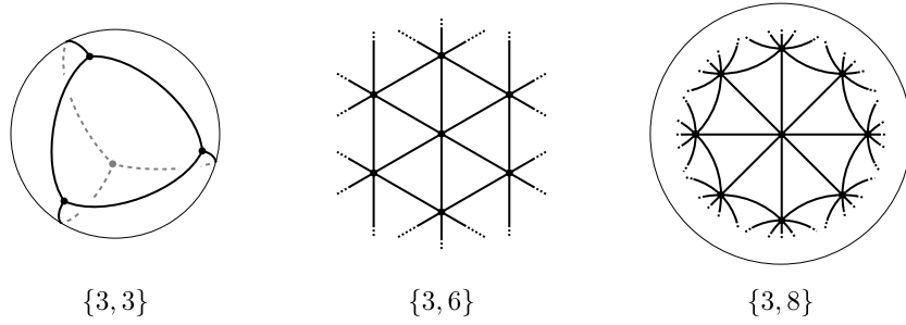
FIGURE 1. Regular tessellations \{3, 3\} , \{3, 6\} and \{3, 8\} , for example
