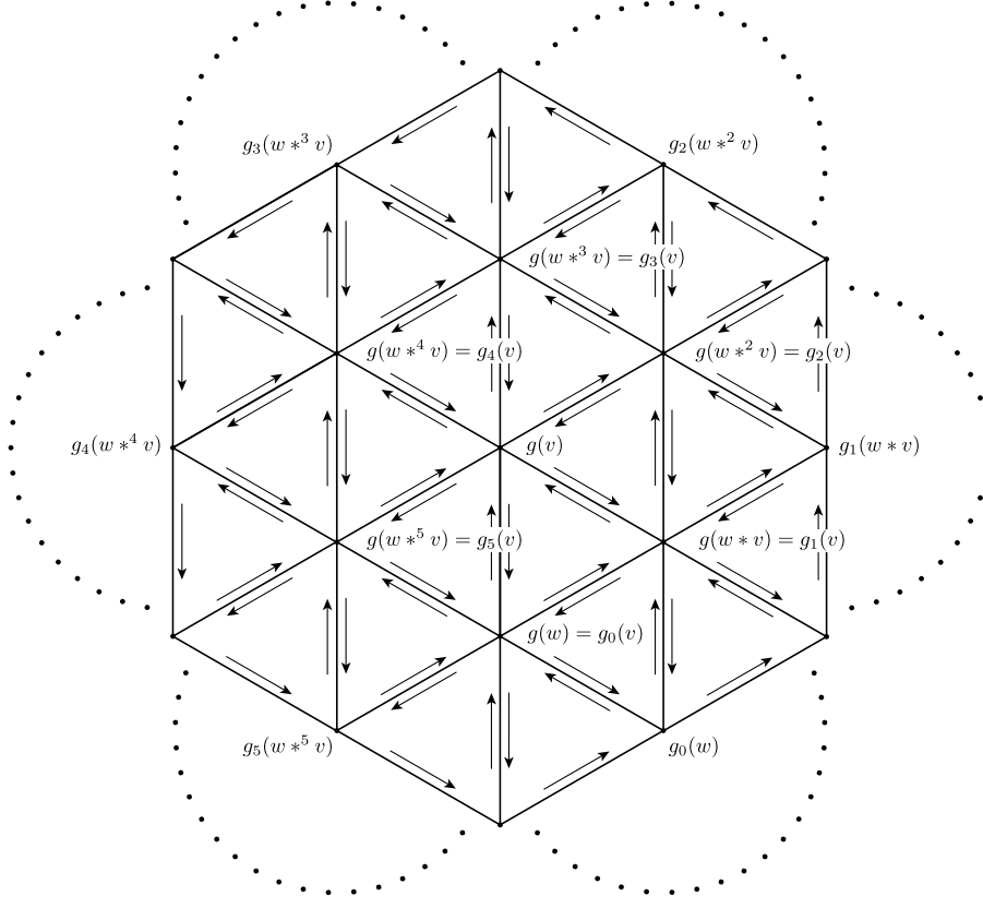
FIGURE 5. A part of the arrangement of triangles (in the case m = 6 )
