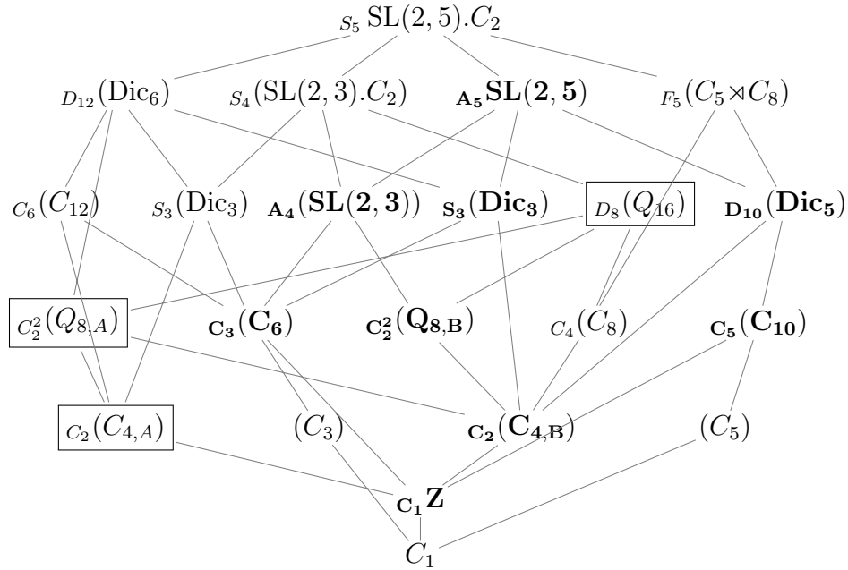
Figure 1: Subgroups of \text{SL}(2, 5).C_2 .
