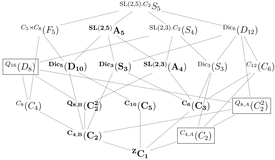
Figure 2: Subgroups of S_5 .
